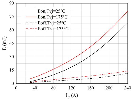
图 9. 开关损耗 Figure 9. Switching losses of IGBT V_{GE}=\pm 15V, R_{gon}=3.3\Omega, R_{goff}=3.3\Omega, V_{CE}=600V
