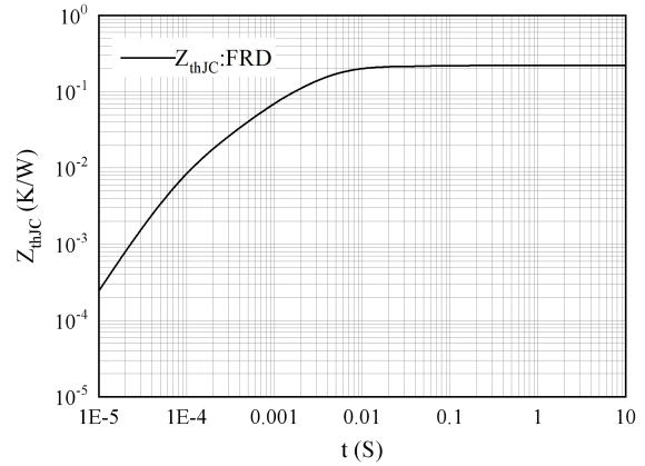
图 8. 瞬态热阻抗 FRD Figure 8. Transient thermal impedance FRD, Z_{thJC}=f(t)
