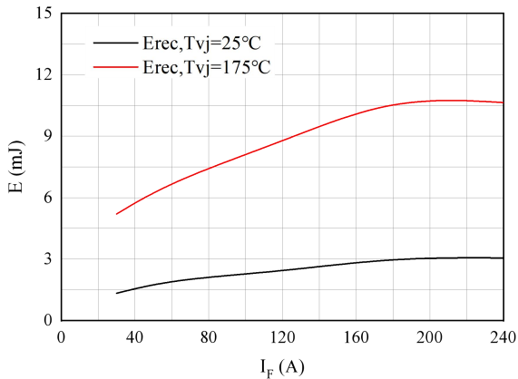
图 11. 开关损耗 二极管 Figure 11. Switching losses of Diode R_{gon}=3.3\Omega, V_{CE}=600V
