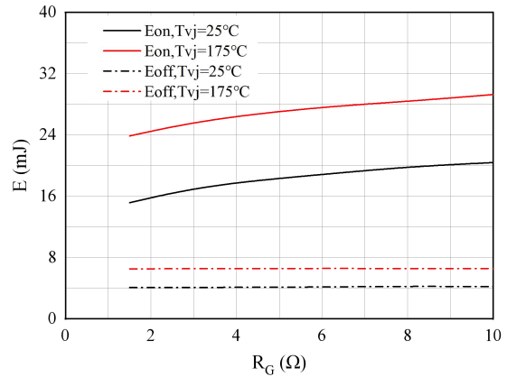
图 10. 开关损耗 Figure 10. Switching losses of IGBT V_{GE}=\pm 15V, I_C=120A, V_{CE}=600V
